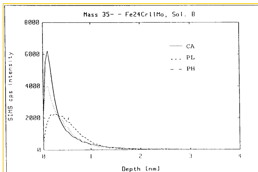
Fig. 15. SIMS intensity-depth profiles of \text{Cl}^- (mass 35) measured on Fe-24Cr and on Fe-24Cr-11Mo polarized at potentials (CA), (PL) and (PH), respectively, in solution B
